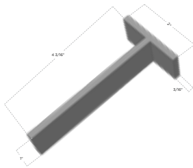
"T" Spacers 1" x 4 3/16" x 2"
